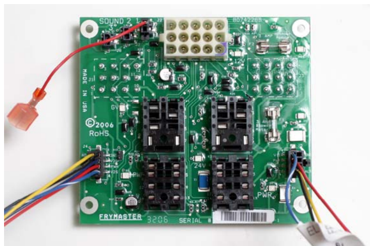
Figure 1: The new H55 service board kit (826-2264) ships with harnesses, which attach the board to the spark module and the sound device.
