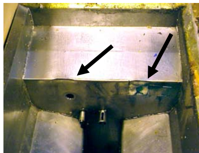
Figure 2: Banging a basket to dislodge oil leads to dents like those shown above. Overtime, hairline cracks can develop and in extreme cases (shown at right) the frypot can be punctured. Such damage is not covered by warranty.
