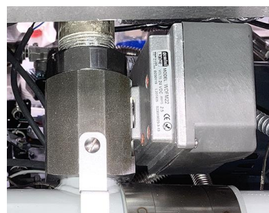
Figure 2 Obsolete Gray Square Actuator attached to drain valve
